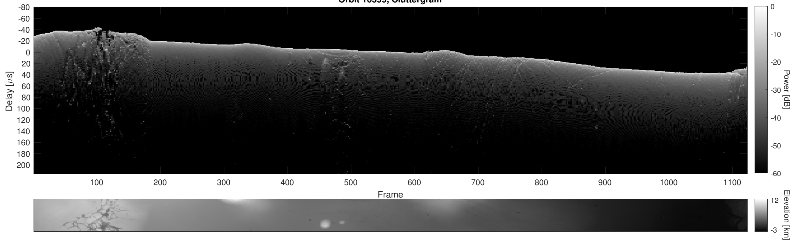
Orbit 16399, Cluttergram
