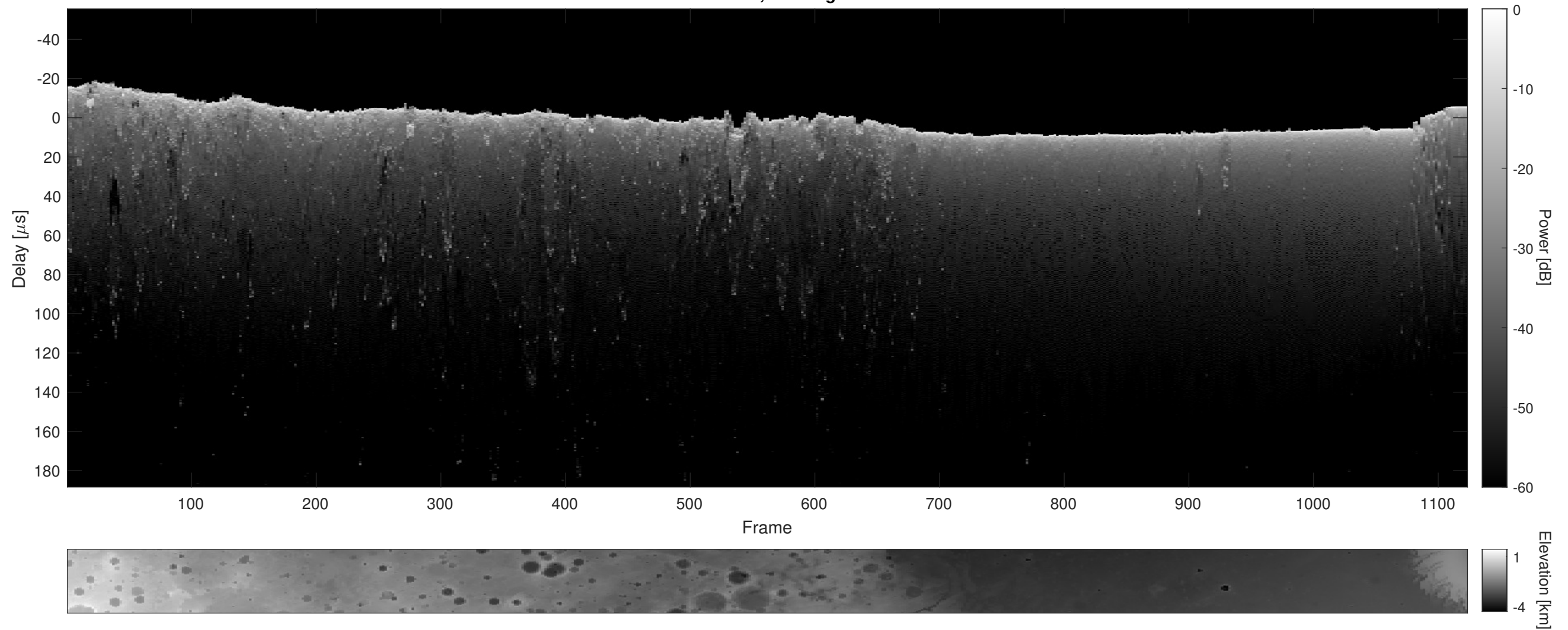
Orbit 16405, Cluttergram
