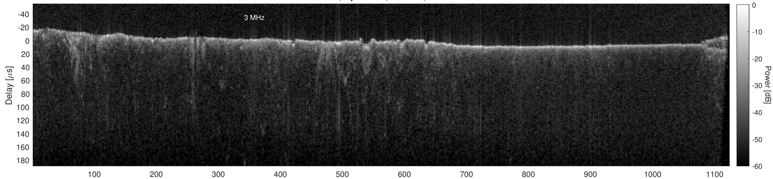
Orbit 16405, Cluttergram
