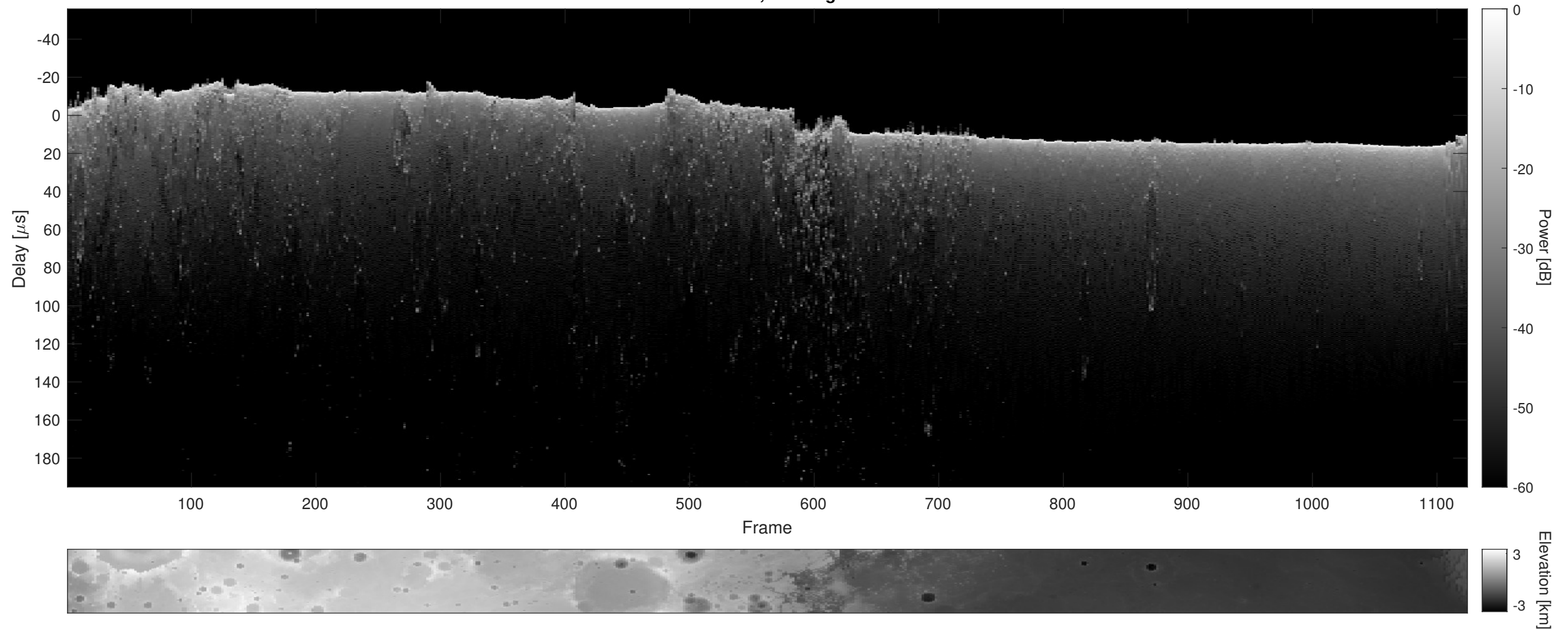
Orbit 16408, Cluttergram
