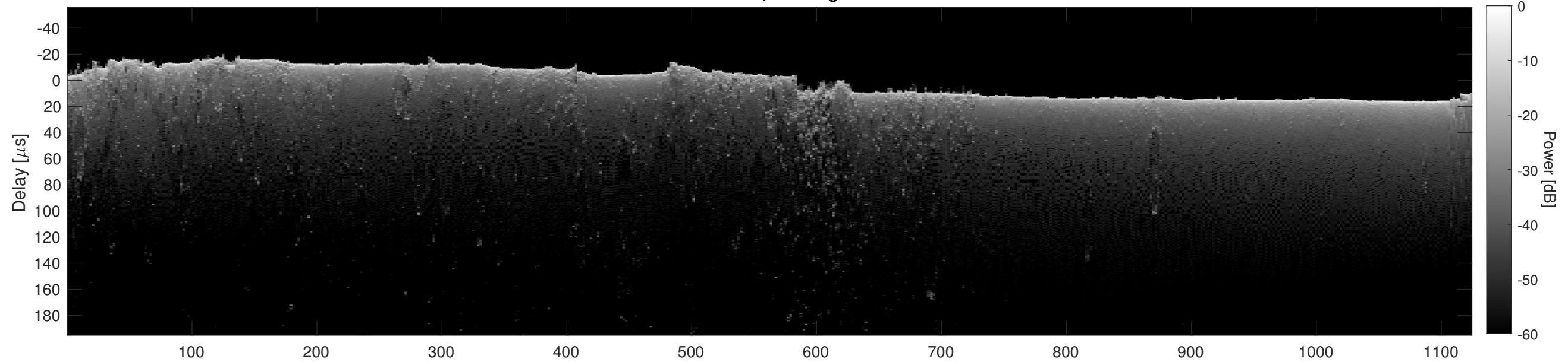
Orbit 16408, Cluttergram
