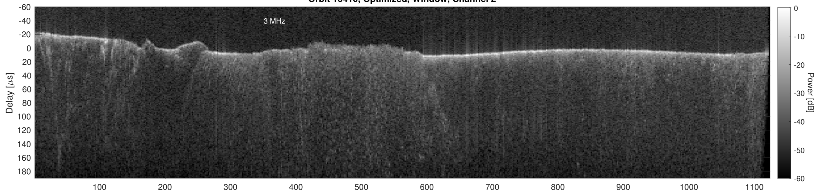
Orbit 16410, Cluttergram
