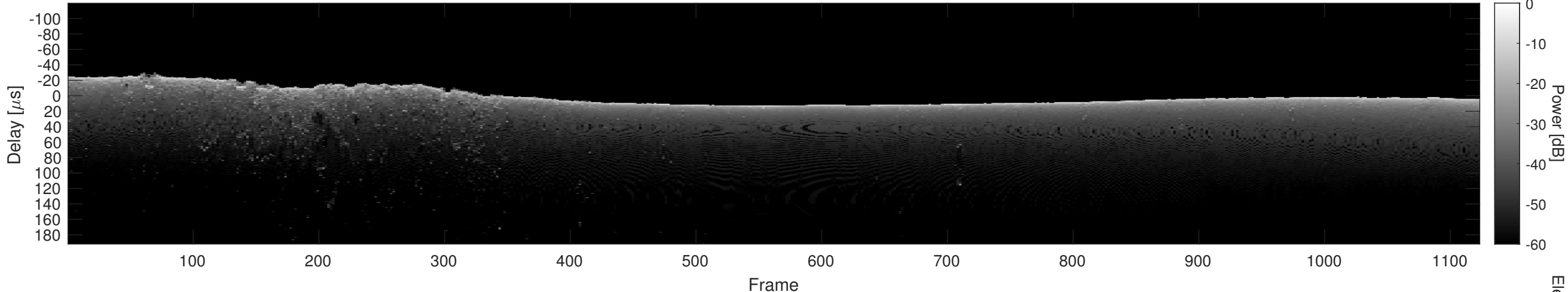
Orbit 16411, Cluttergram
