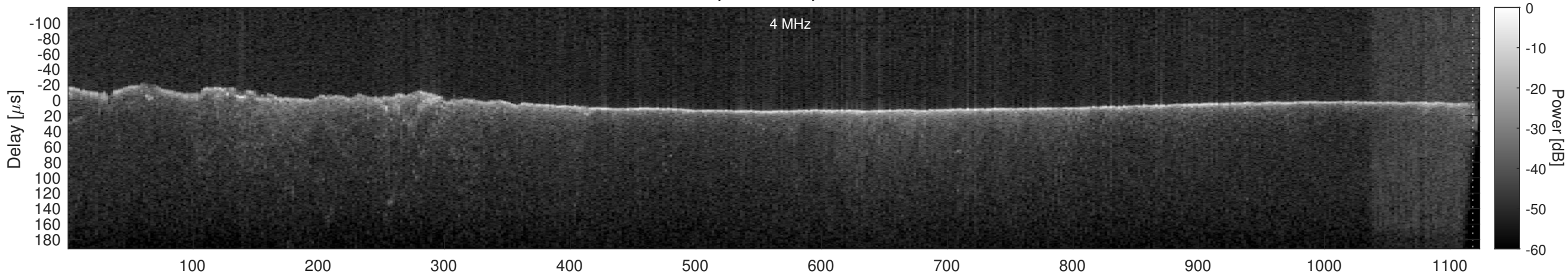
Orbit 16411, Window, Channel 1, Chapman
