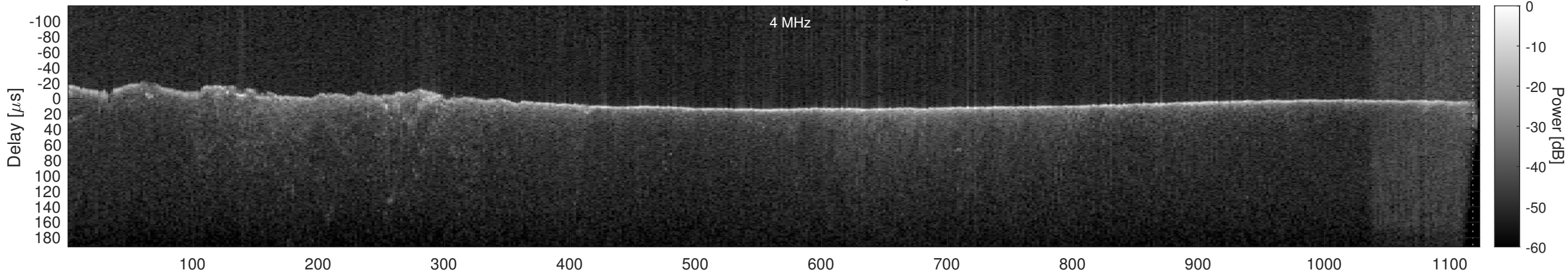
Orbit 16411, Window, Channel 1, Optimized
