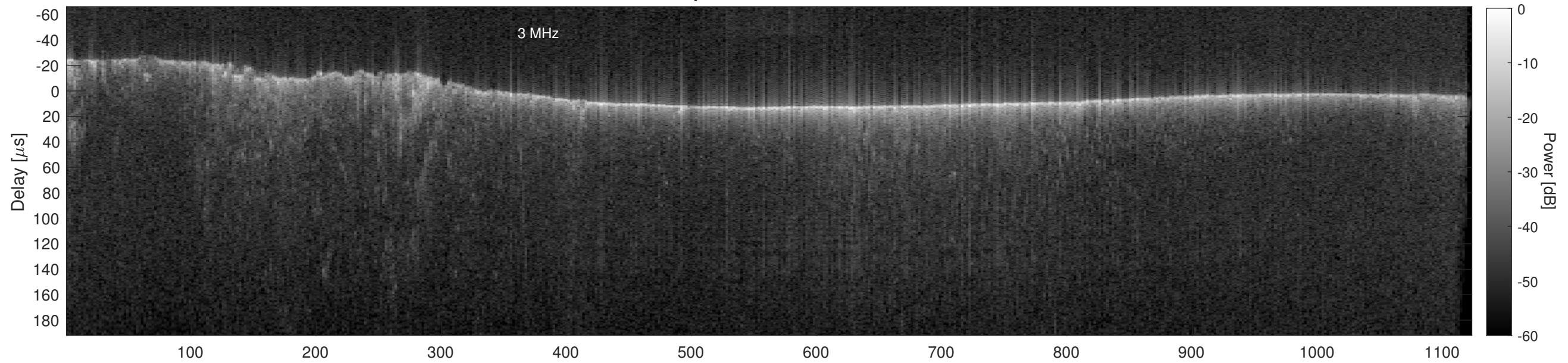
Orbit 16411, Cluttergram
