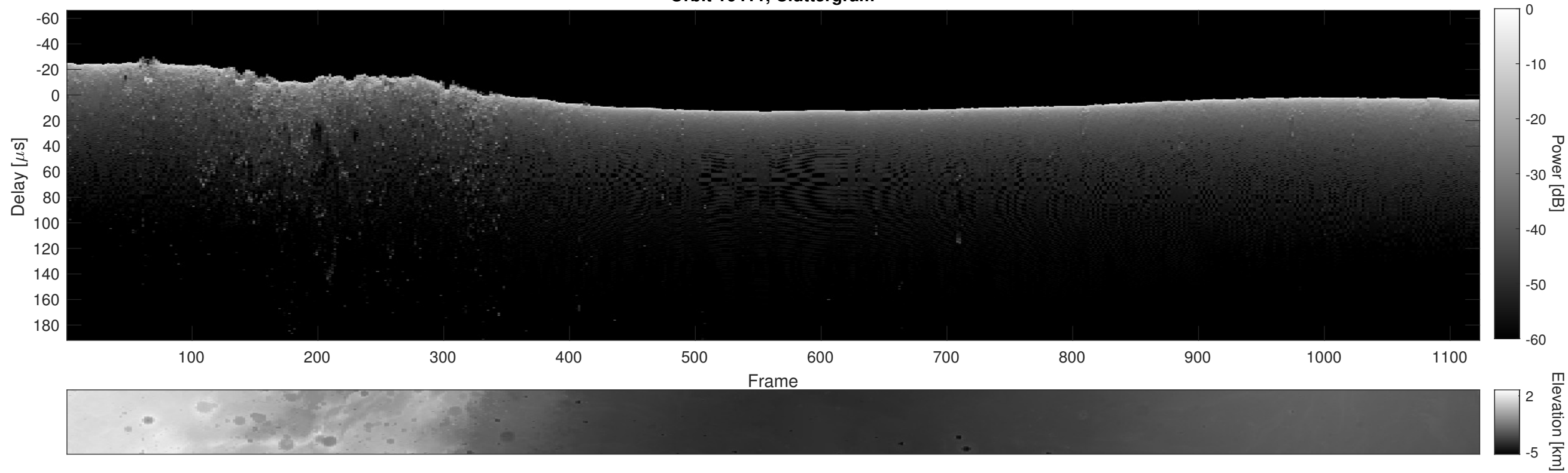
Orbit 16411, Cluttergram
