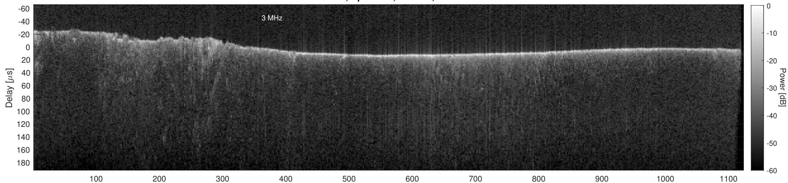
Orbit 16411, Cluttergram
