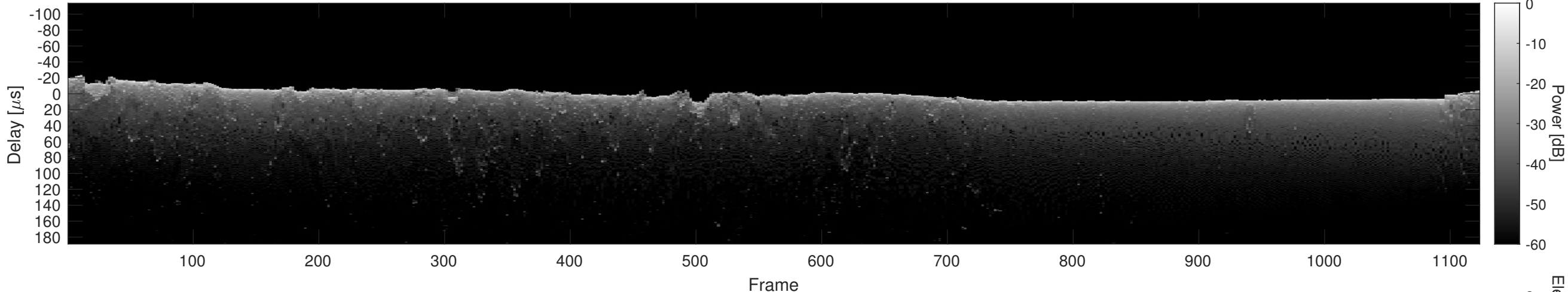
Orbit 16412, Cluttergram
