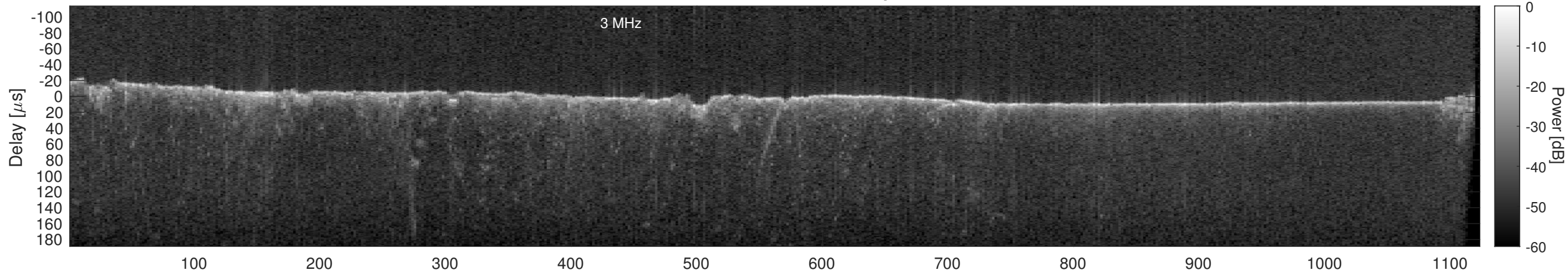
Orbit 16412, Cluttergram
