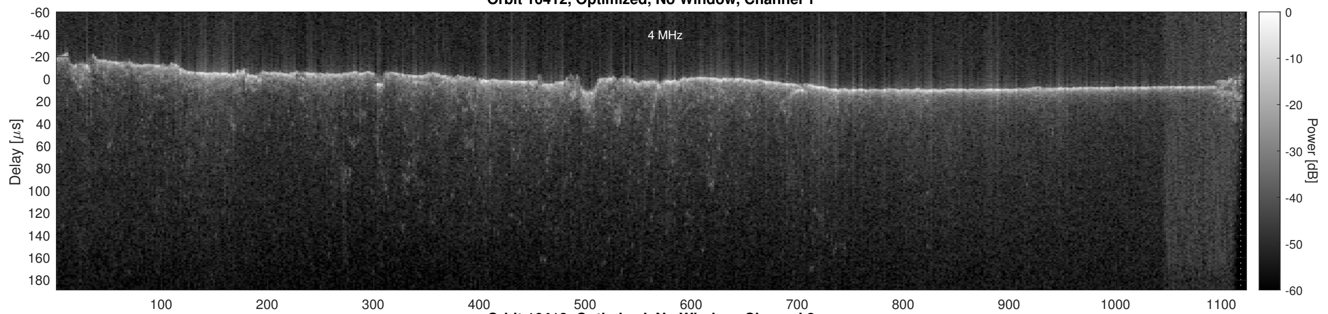
Orbit 16412, Optimized, No Window, Channel 2
