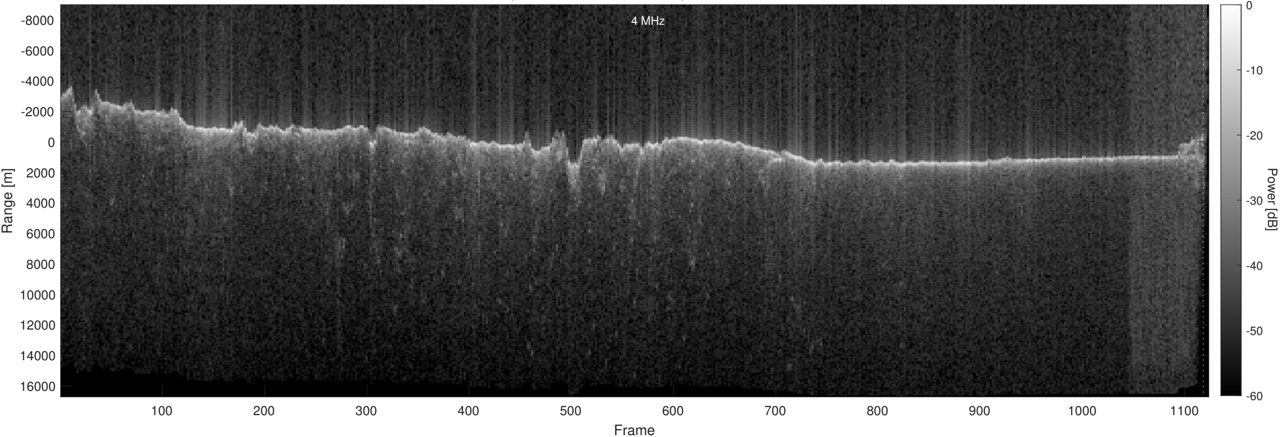
Orbit 16412, Optimized, No Window, Depth-Corrected, Channel 2
