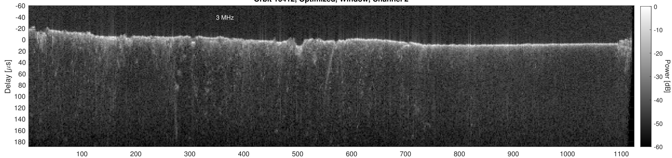
Orbit 16412, Cluttergram
