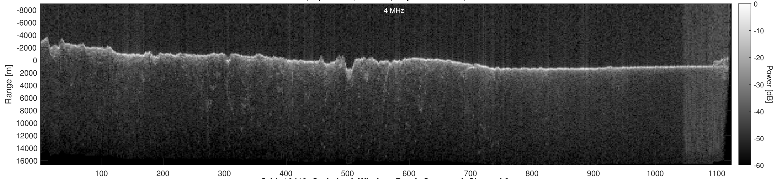
Orbit 16412, Optimized, Window, Depth-Corrected, Channel 2
