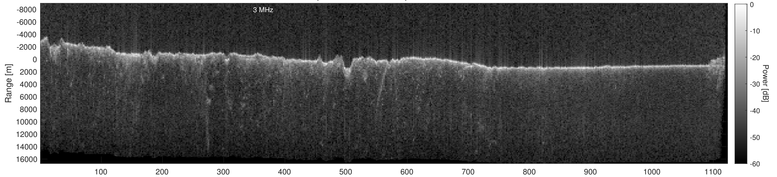
Orbit 16412, Depth-Corrected Cluttergram
