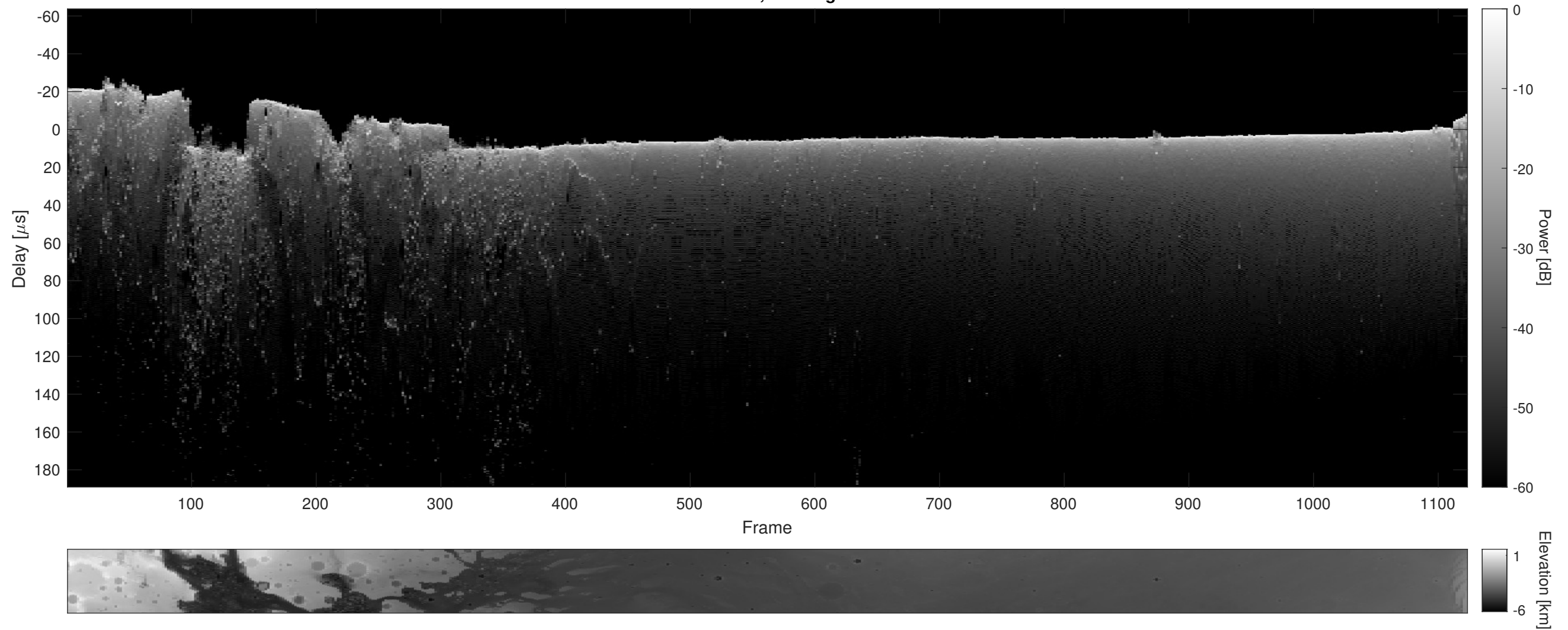
Orbit 16416, Cluttergram
