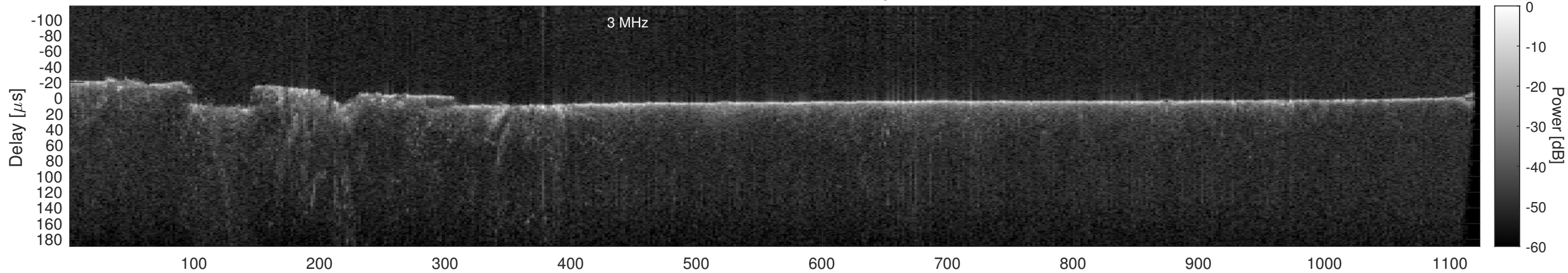
Orbit 16416, Cluttergram
