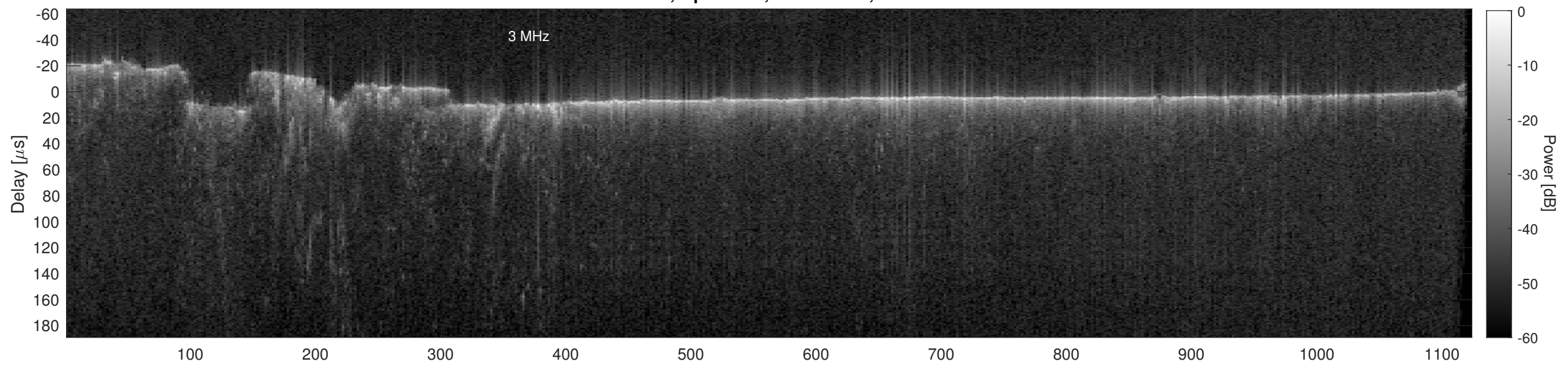
Orbit 16416, Cluttergram
