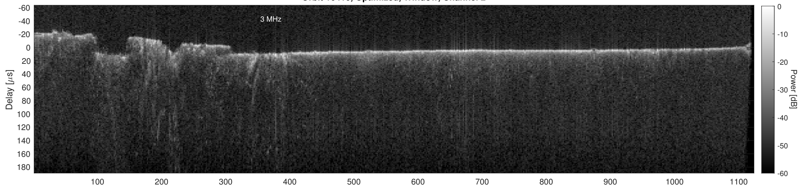
Orbit 16416, Cluttergram
