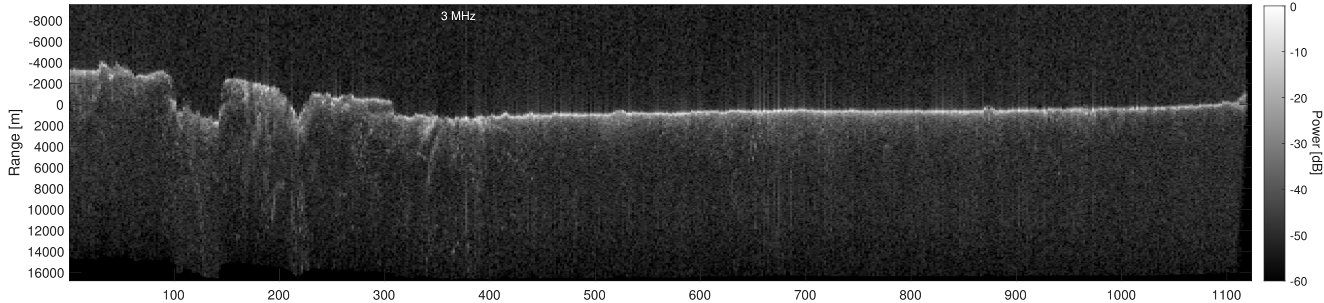
Orbit 16416, Depth-Corrected Cluttergram
