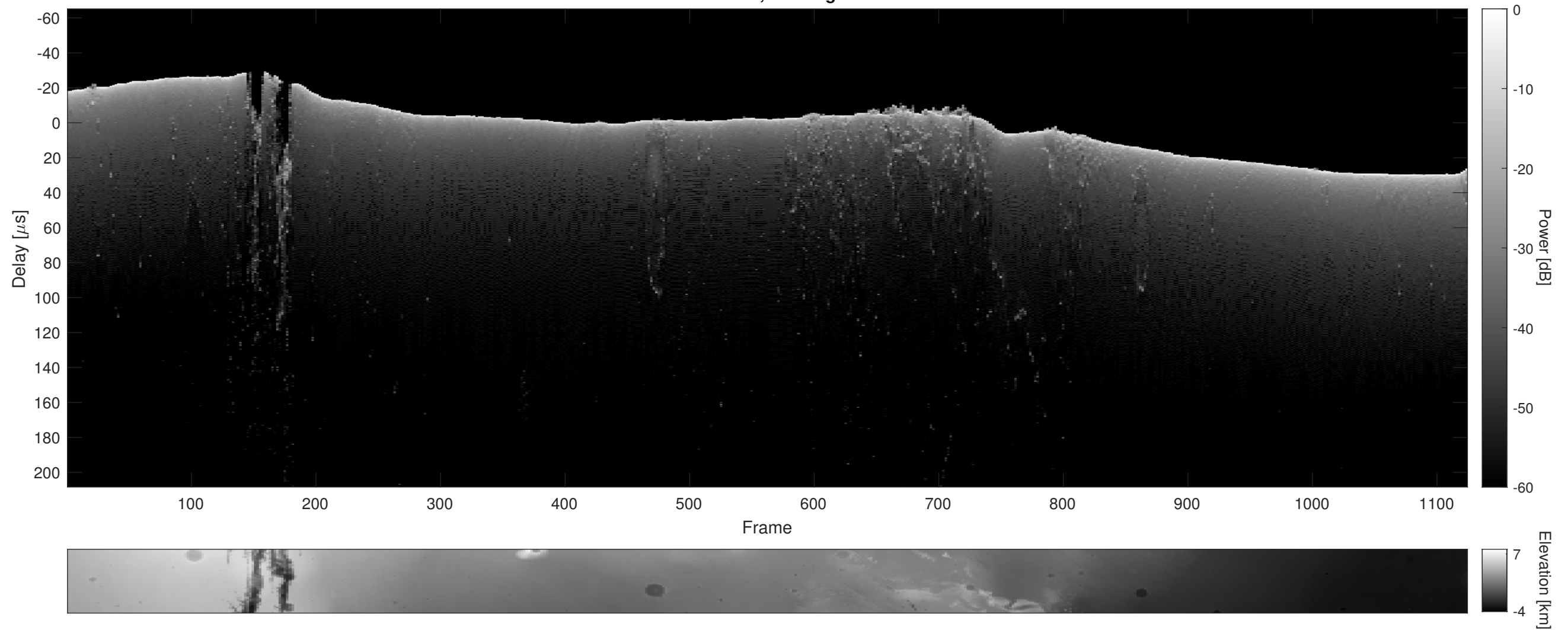
Orbit 16420, Cluttergram
