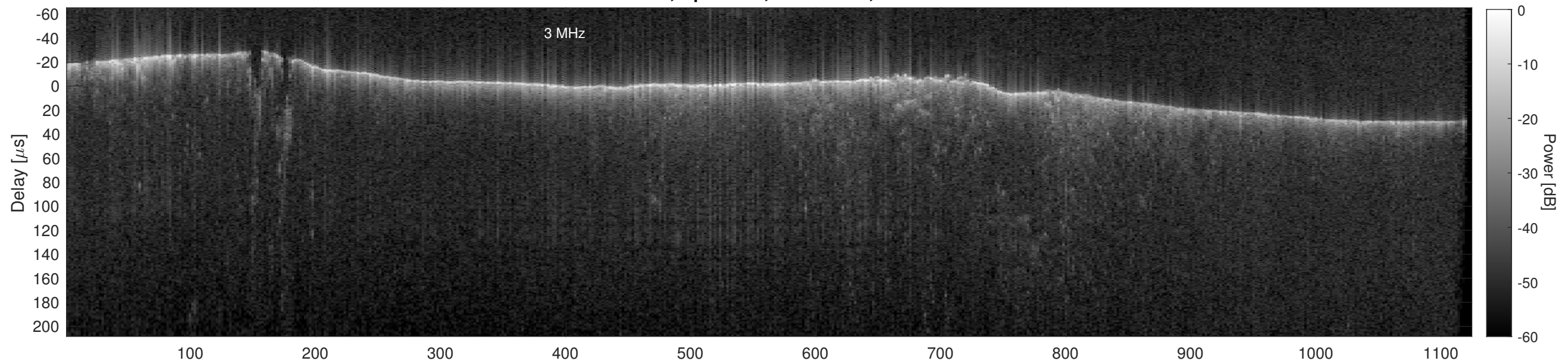
Orbit 16420, Cluttergram
