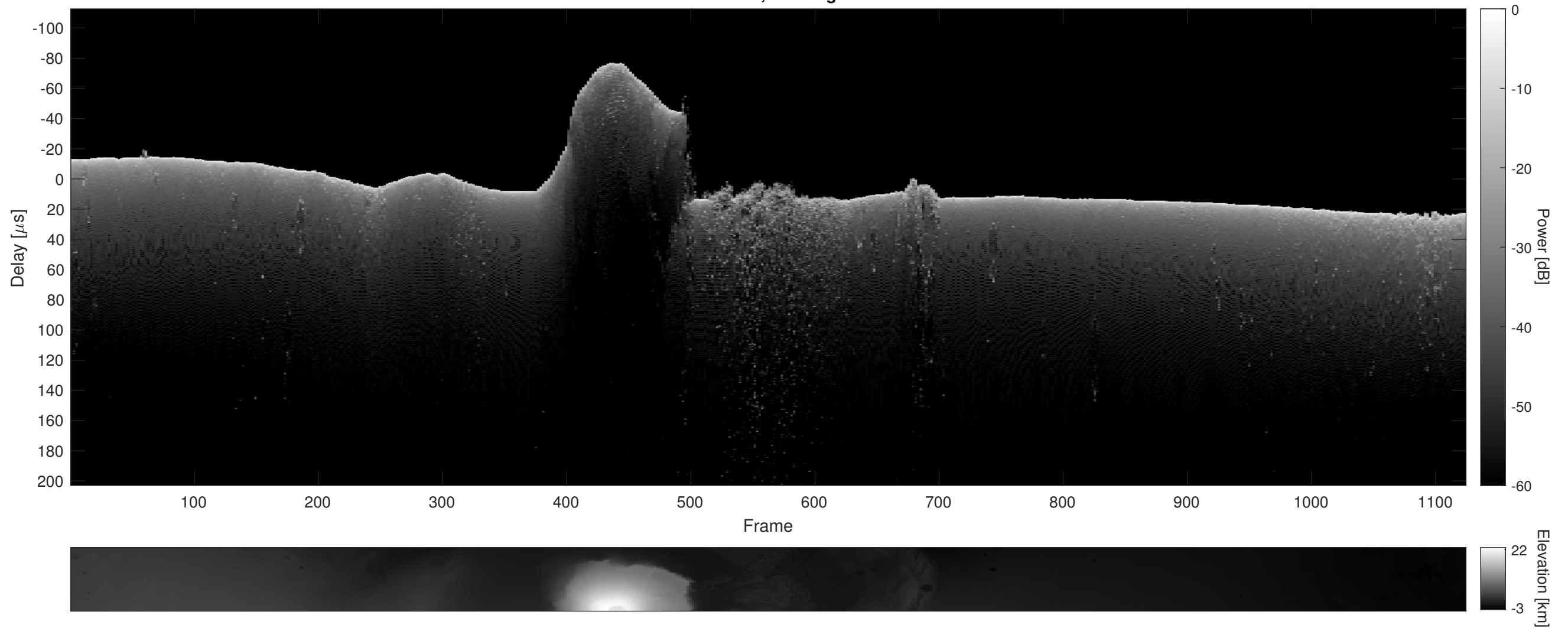
Orbit 16424, Cluttergram
