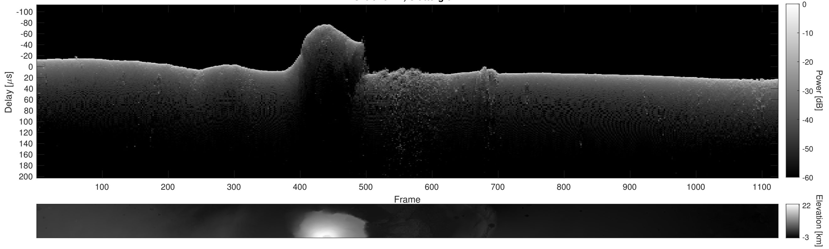
Orbit 16424, Cluttergram
