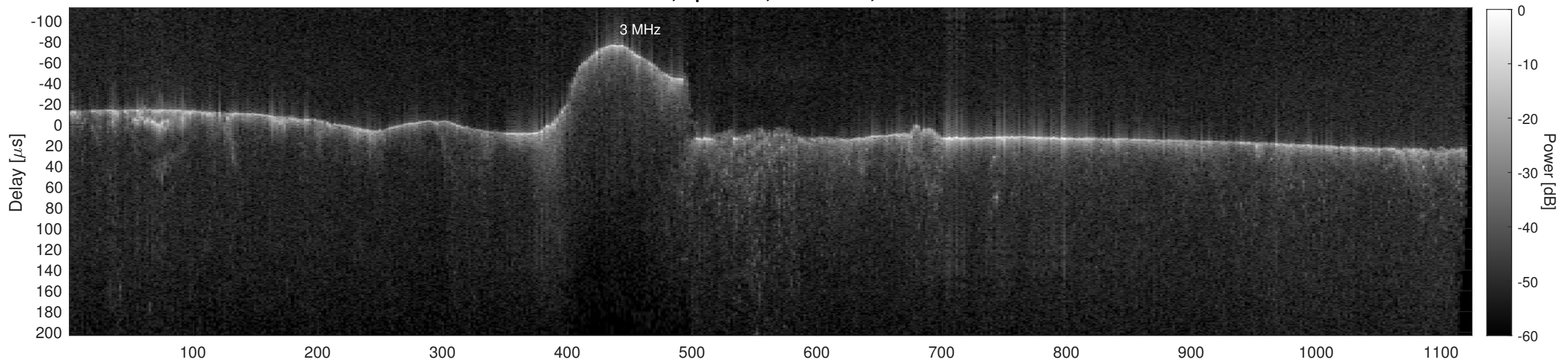
Orbit 16424, Cluttergram
