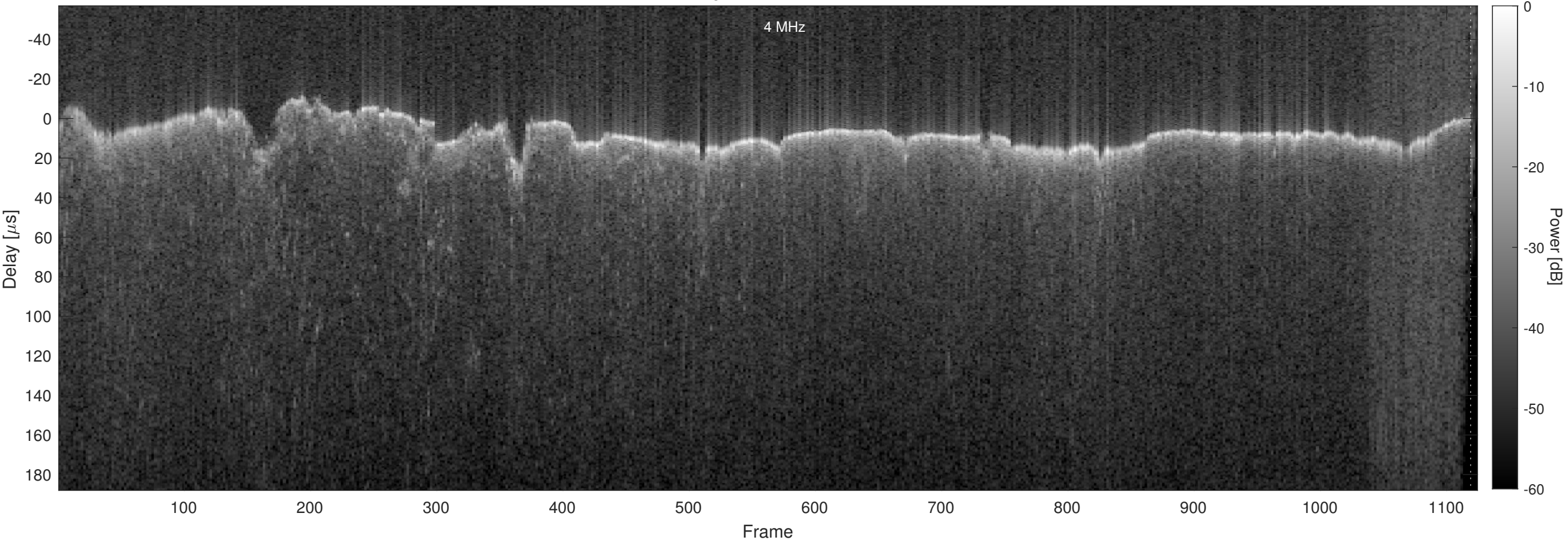
Orbit 16430, Chapman, No Window, Channel 2
