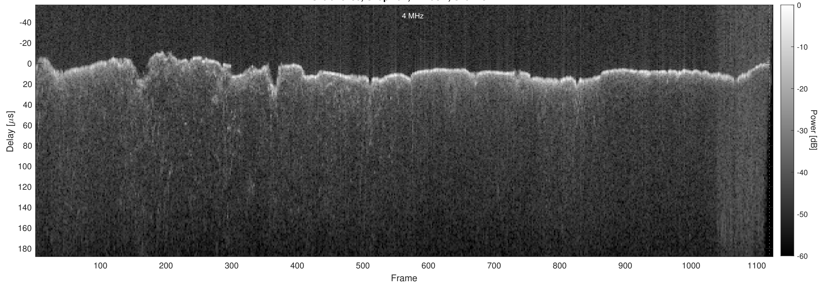
Orbit 16430, Chapman, Window, Channel 2
