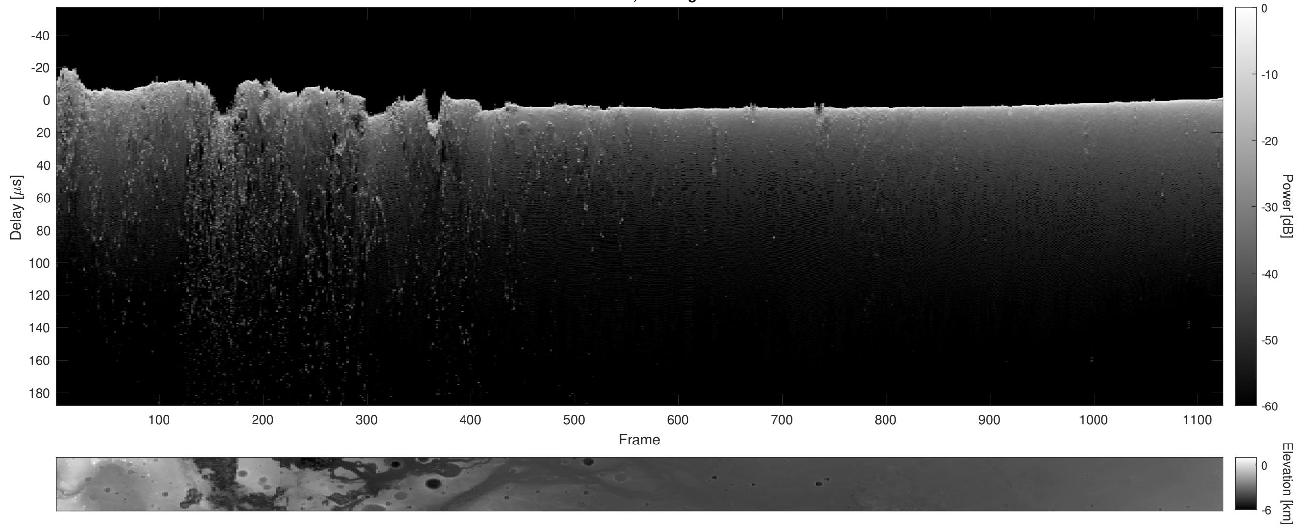
Orbit 16430, Cluttergram
