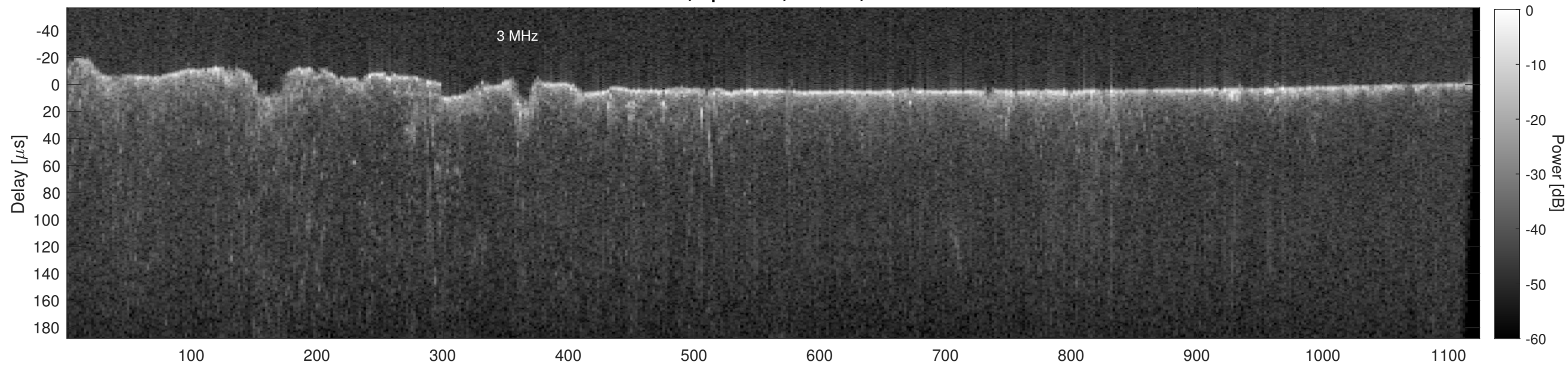
Orbit 16430, Cluttergram
