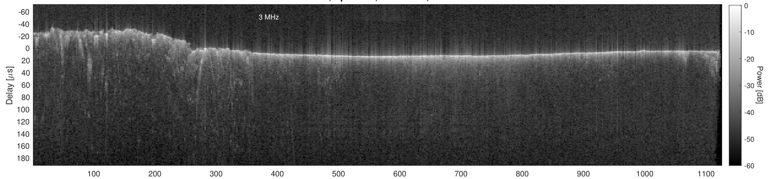
Orbit 16432, Cluttergram
