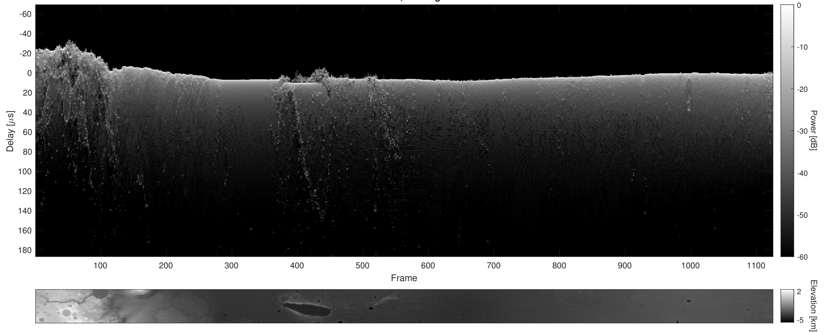
Orbit 16435, Cluttergram
