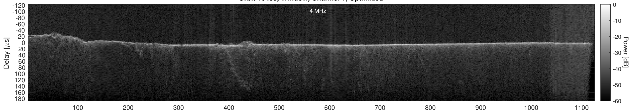
Orbit 16435, Cluttergram
