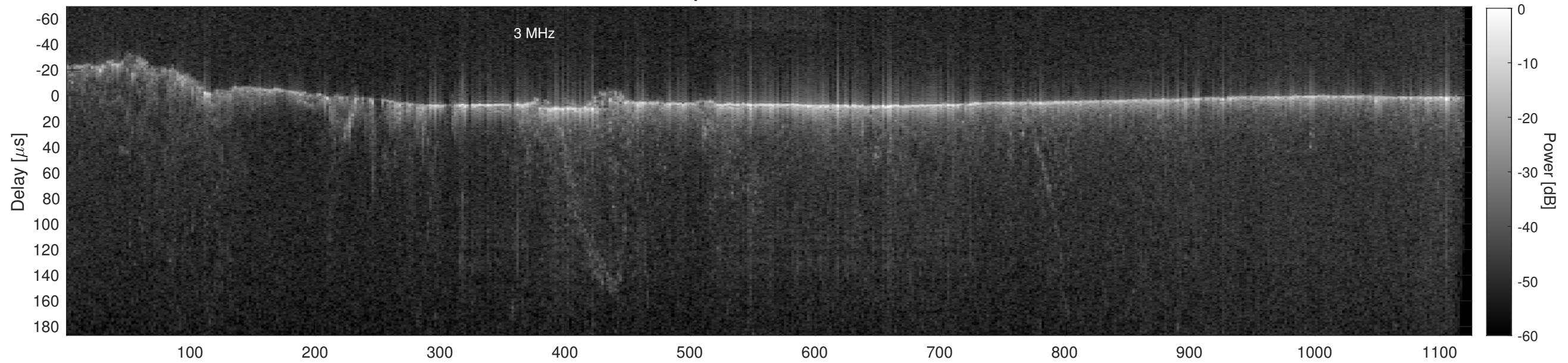
Orbit 16435, Cluttergram
