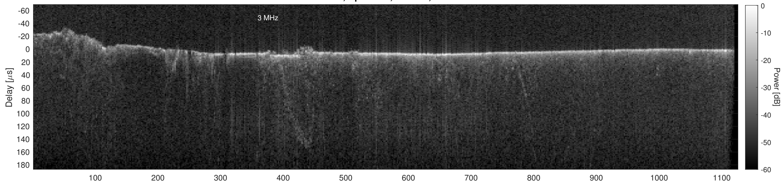
Orbit 16435, Cluttergram
