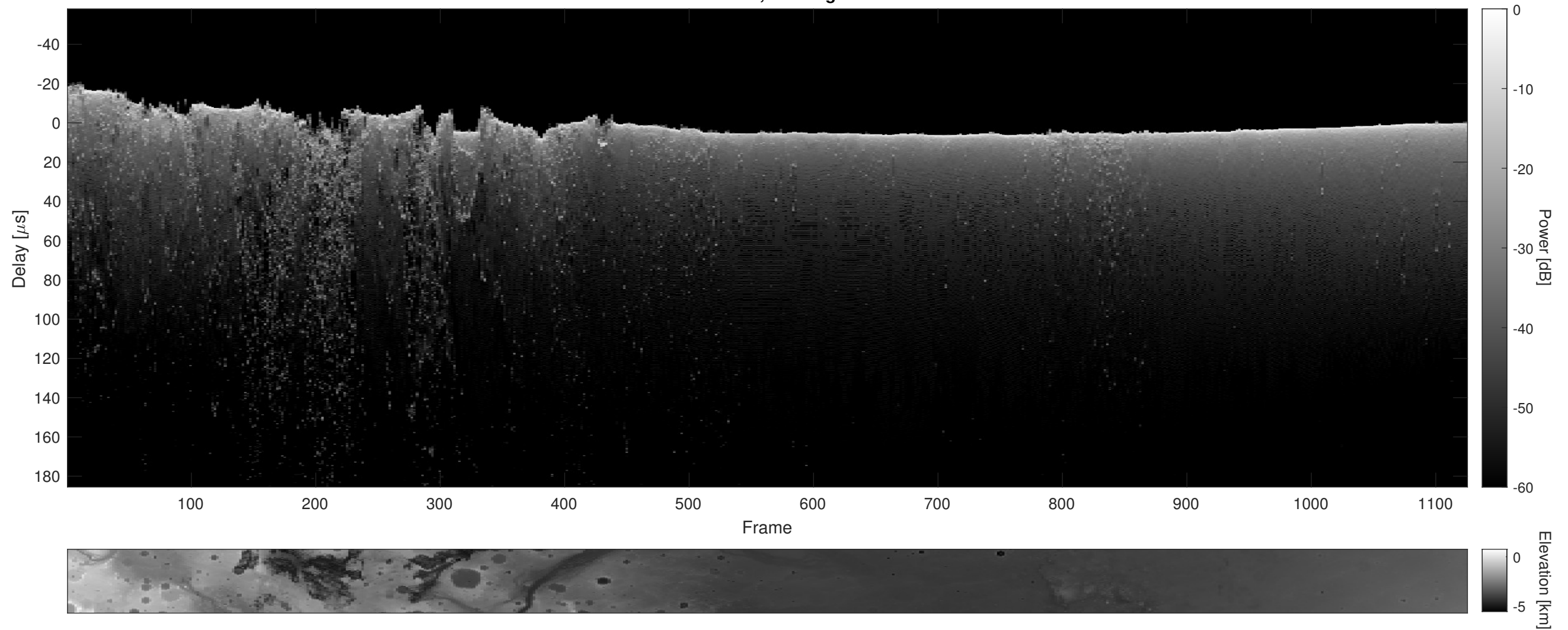
Orbit 16437, Cluttergram
