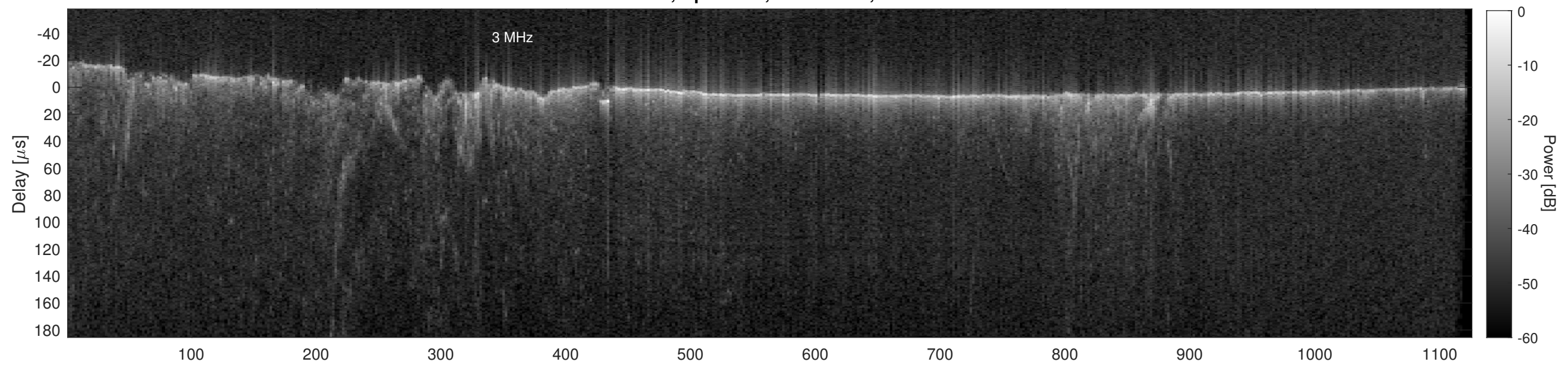
Orbit 16437, Cluttergram
