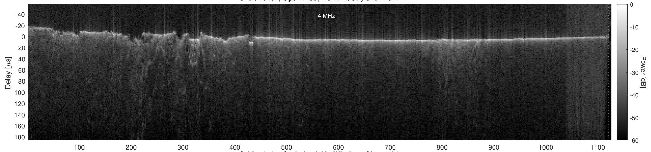
Orbit 16437, Optimized, No Window, Channel 2
