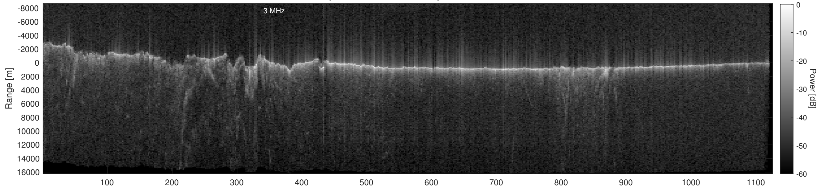
Orbit 16437, Depth-Corrected Cluttergram
