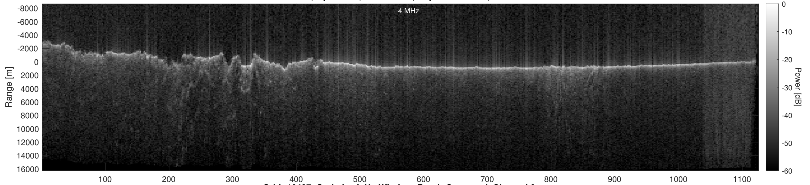
Orbit 16437, Optimized, No Window, Depth-Corrected, Channel 2
