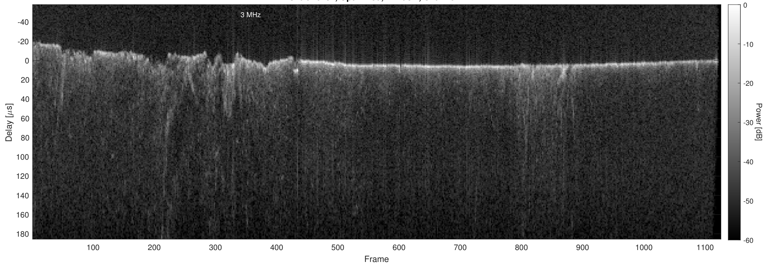
Orbit 16437, Optimized, Window, Channel 2
