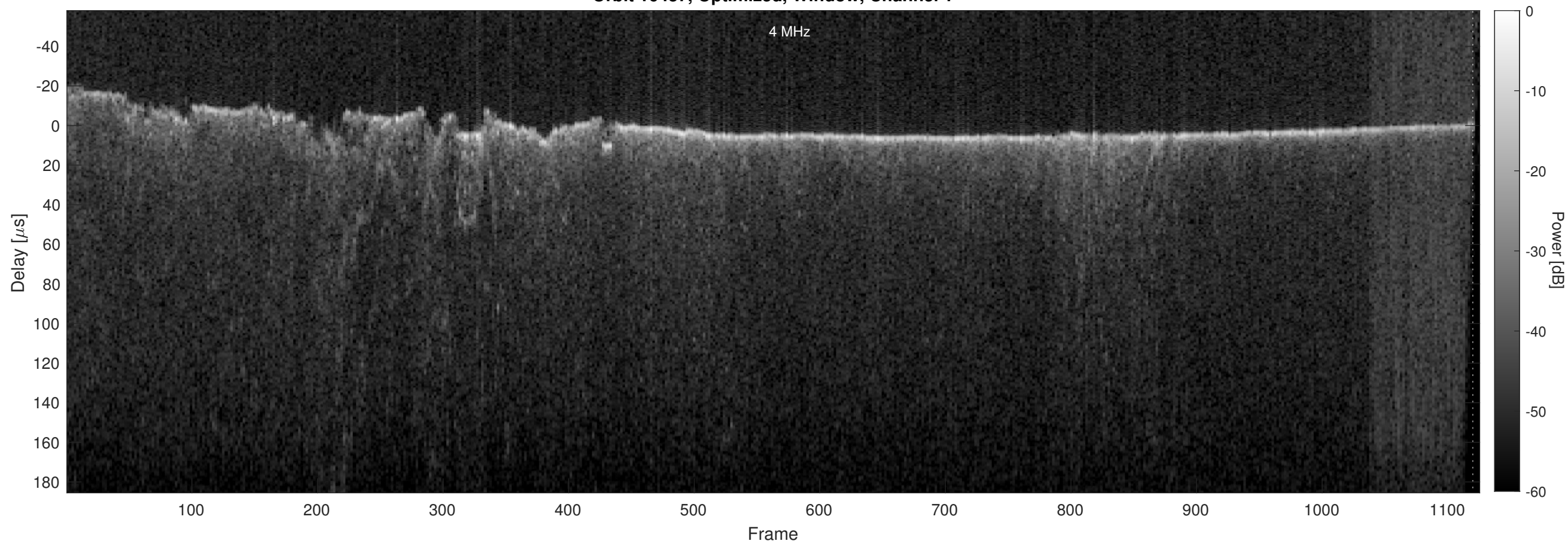
Orbit 16437, Optimized, Window, Channel 2
