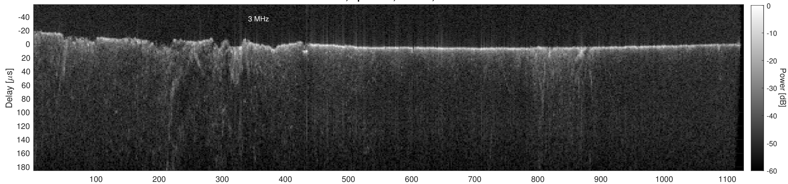
Orbit 16437, Cluttergram
