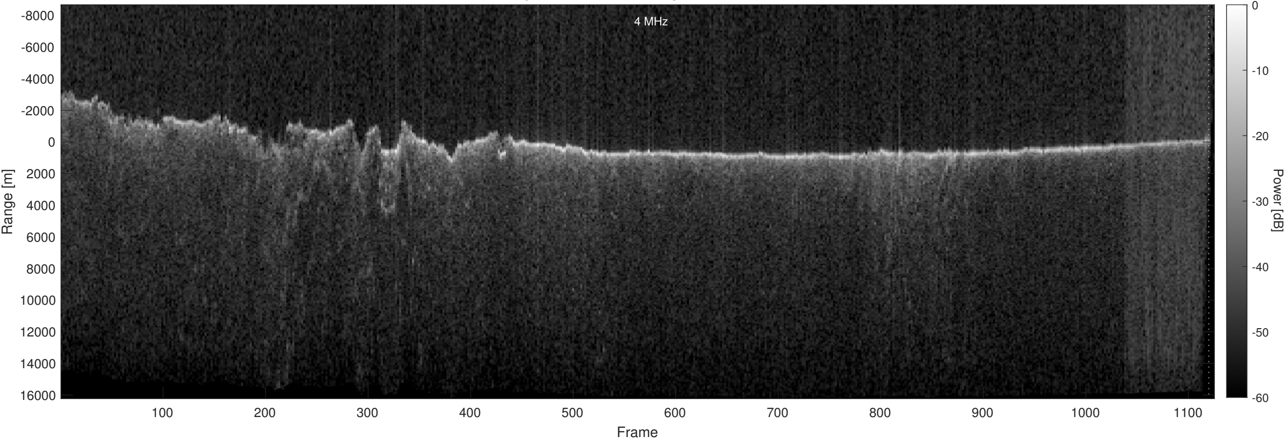
Orbit 16437, Optimized, Window, Depth-Corrected, Channel 2
