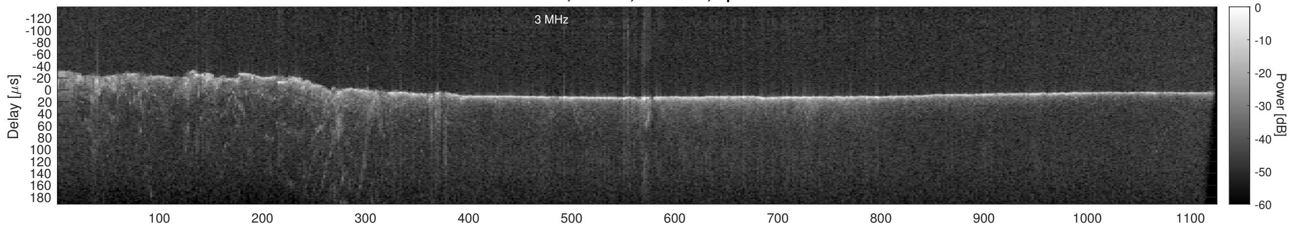
Orbit 16439, Cluttergram
