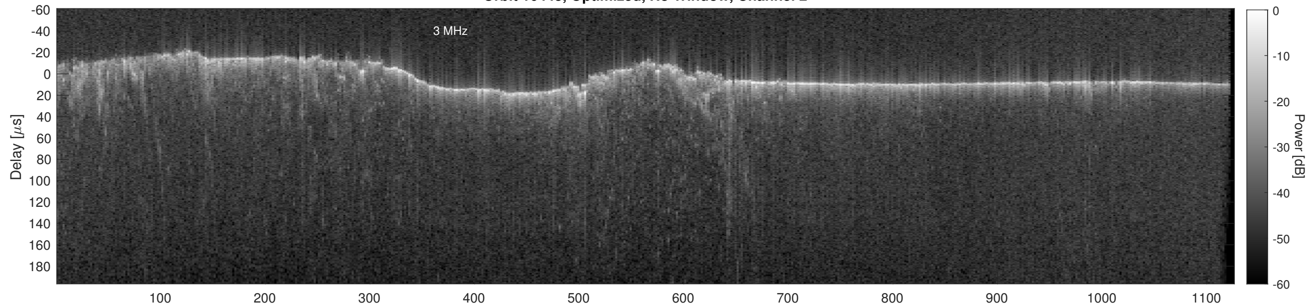
Orbit 16443, Cluttergram
