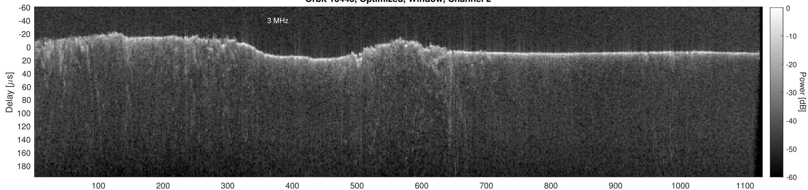
Orbit 16443, Cluttergram
