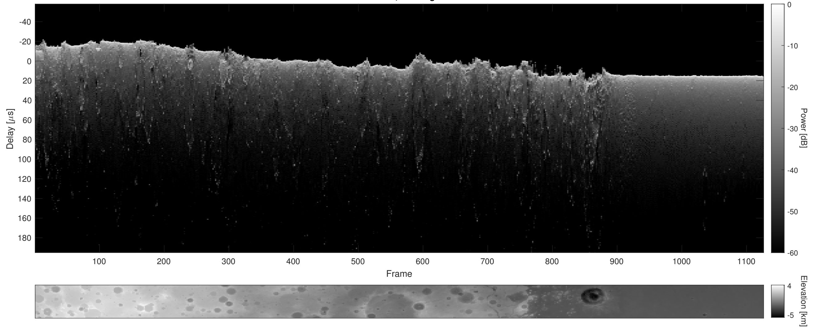
Orbit 16447, Cluttergram
