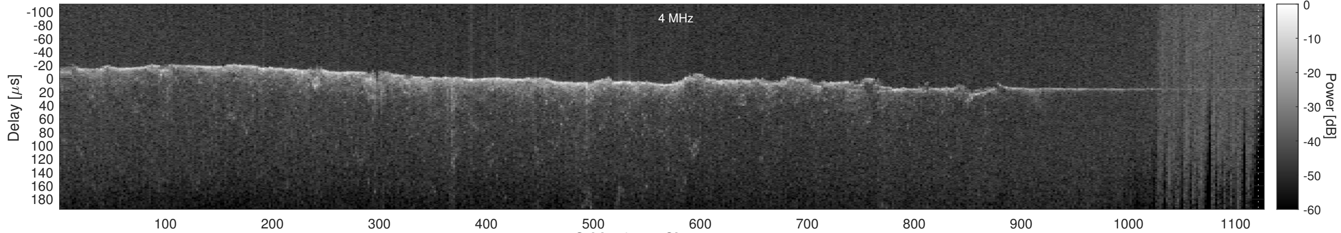
Orbit 16447, Cluttergram
