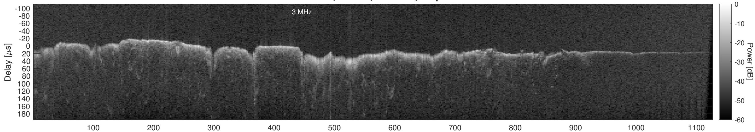
Orbit 16447, Window, Channel 2, Optimized
