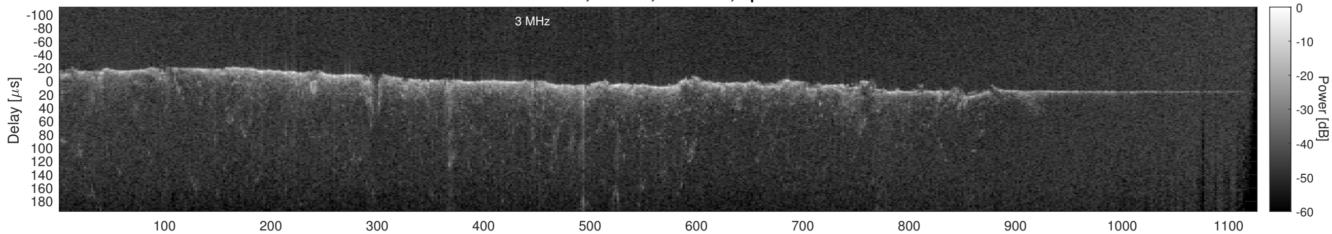
Orbit 16447, Cluttergram
