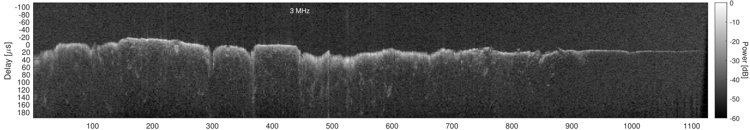
Orbit 16447, Window, Channel 2, Chapman
