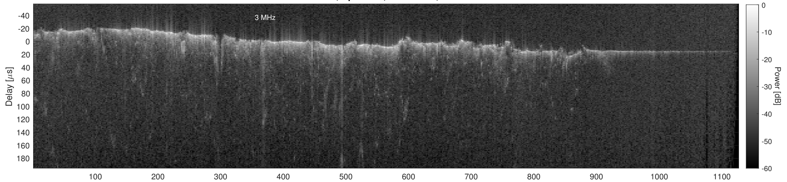
Orbit 16447, Cluttergram
