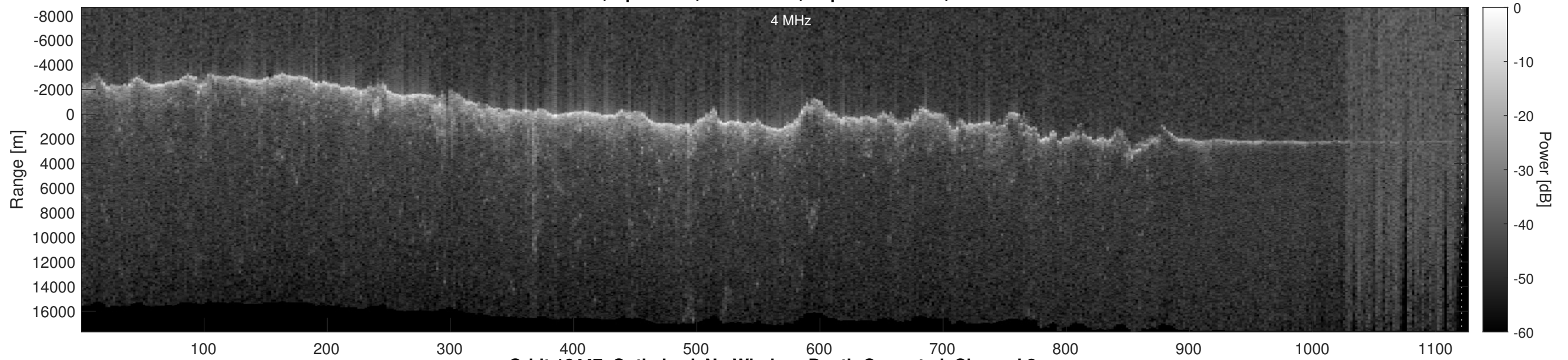
Orbit 16447, Optimized, No Window, Depth-Corrected, Channel 2
