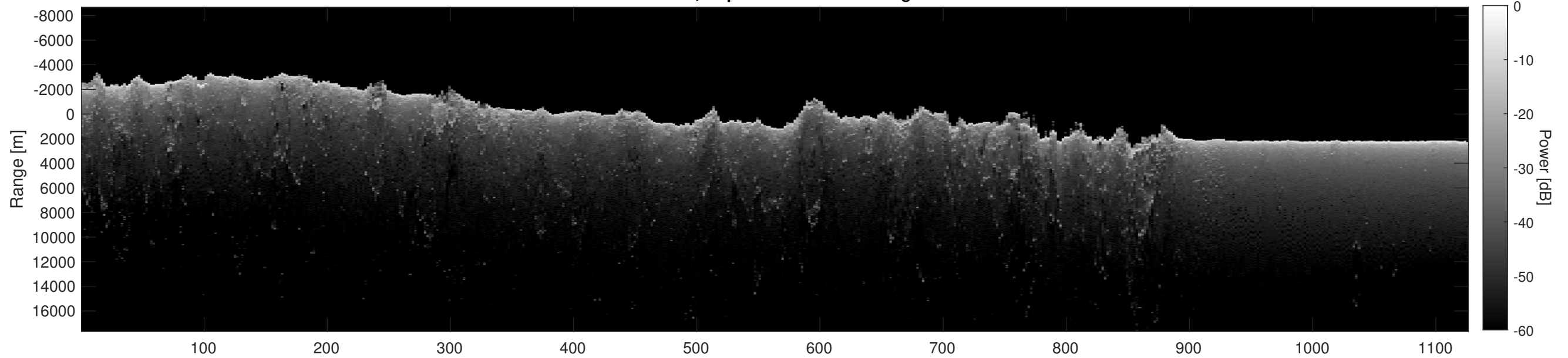
Orbit 16447, Depth-Corrected Cluttergram
