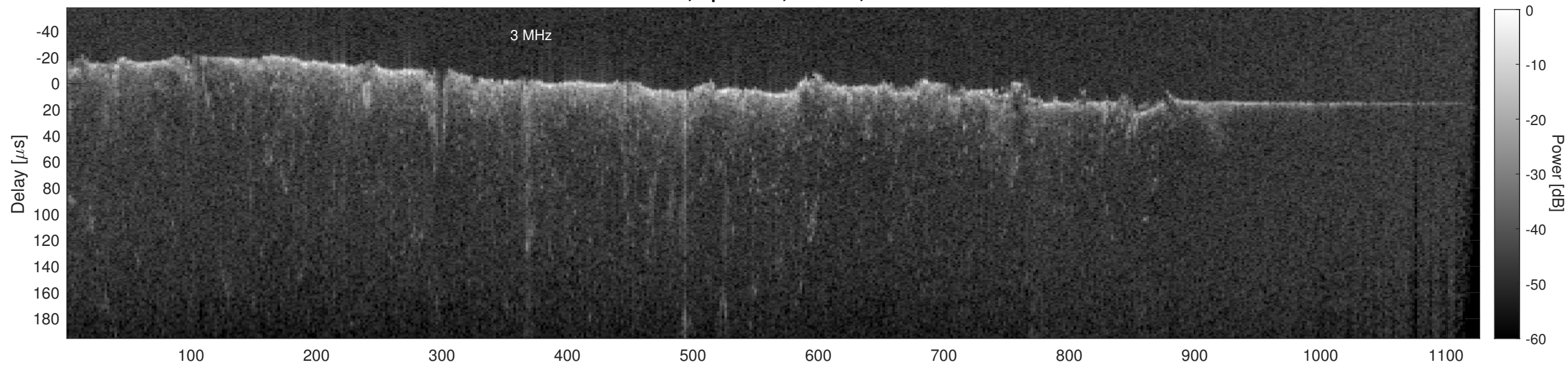
Orbit 16447, Cluttergram
