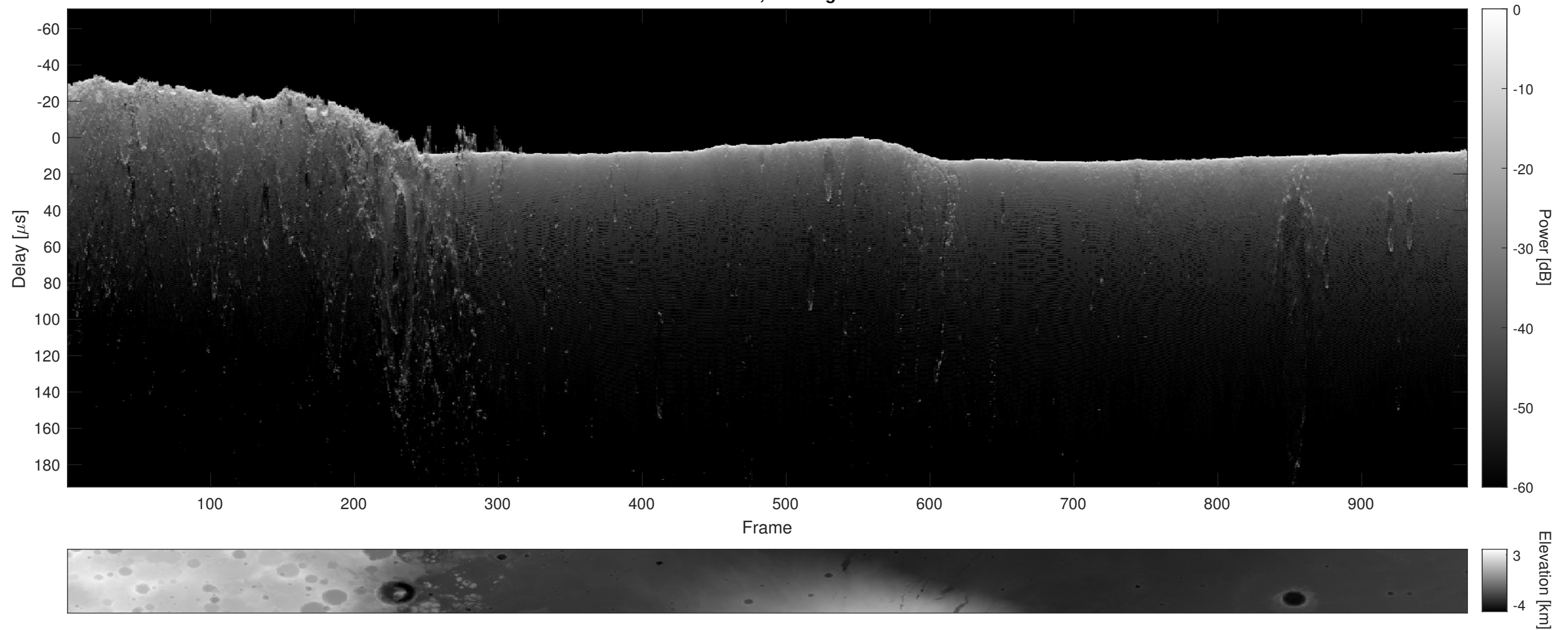
Orbit 16453, Cluttergram
