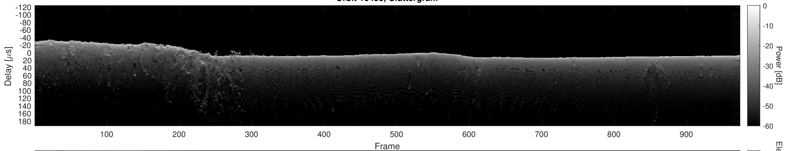
Orbit 16453, Cluttergram
