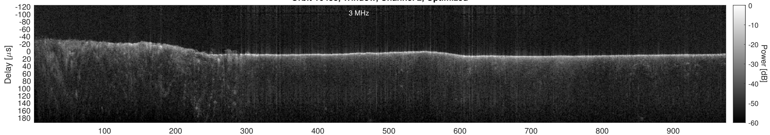
Orbit 16453, Cluttergram
